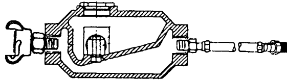
WHIP HOSE/LUBRICATOR ASSY. 9095-4 Hose, 9371 Lubricator (Hose 1/2" I/D X 10 Foot)
