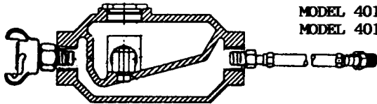
WHIP HOSE/LUBRICATOR ASSY. 9095-4 Hose, 9371 Lubricator (Hose 1/2" I/D X 10 Foot)
